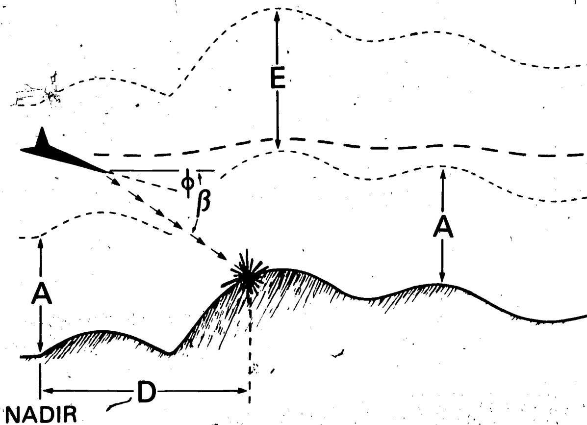
FIGURE 1 Depiction of low level flight task. A = minimum altitude above ground; \beta = flight path angle; \phi = pitch angle (attitude). Cross-hatching indicates desired flightband; heavy dashed line is minimal flight path.
